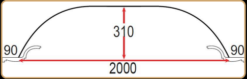
PVT23 D: 2000mm
